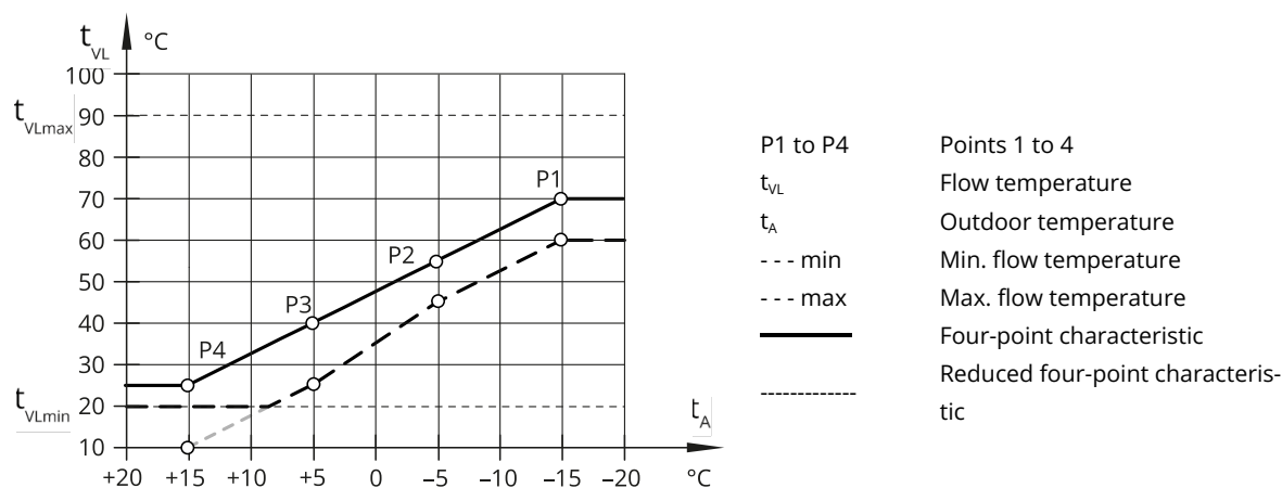
Fig. 16: Four-point characteristic
