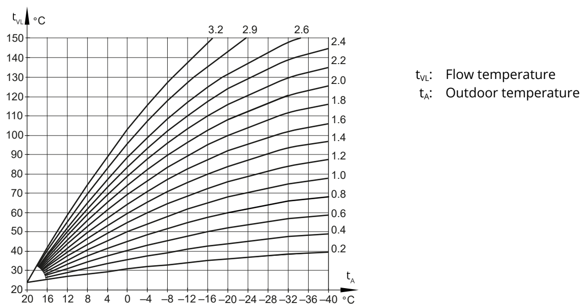
Fig. 15: Gradient characteristics
