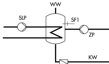
Fig. 17: Schematics of a storage tank system
