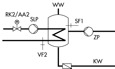
Fig. 18: Schematics of a storage tank system with a globe valve for return temperature limitation
