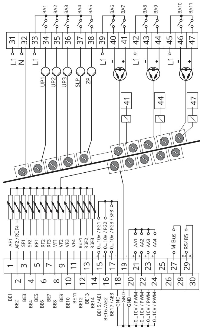
Fig. 3: Electrical connection · TROVIS 5578-1113
