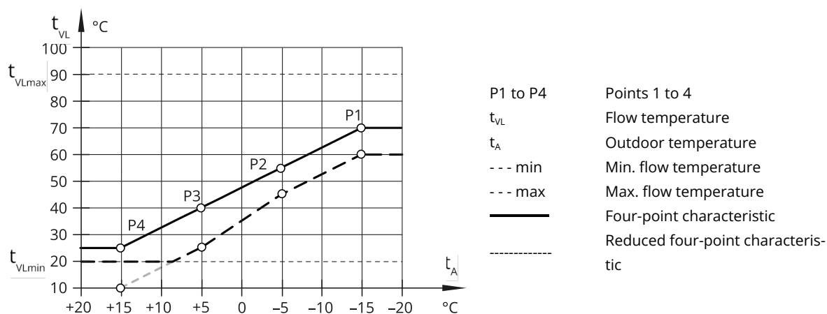
Fig. 16: Four-point characteristic
