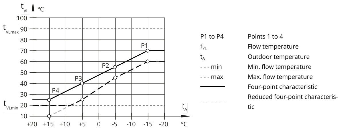
Fig. 16: Four-point characteristic
