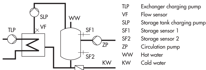
Fig. 10 · Schematics of a storage tank charging system
