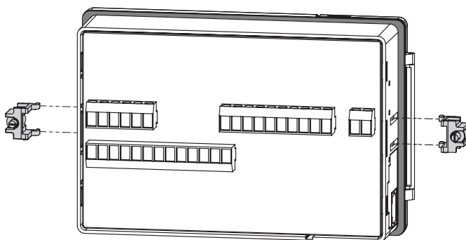
Fig. 8 · Panel mounting
