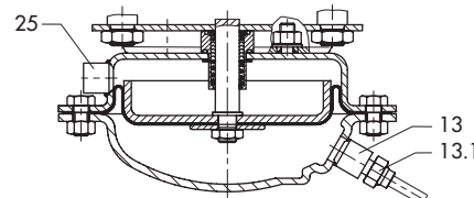
Actuator with leakage line connection
