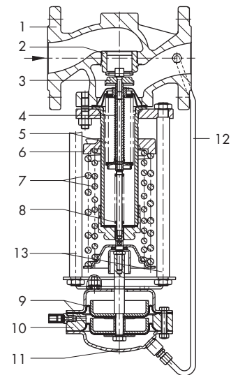
Type 36-3 Pressure Reducing Valve
