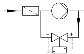
Einbau in Bypass
