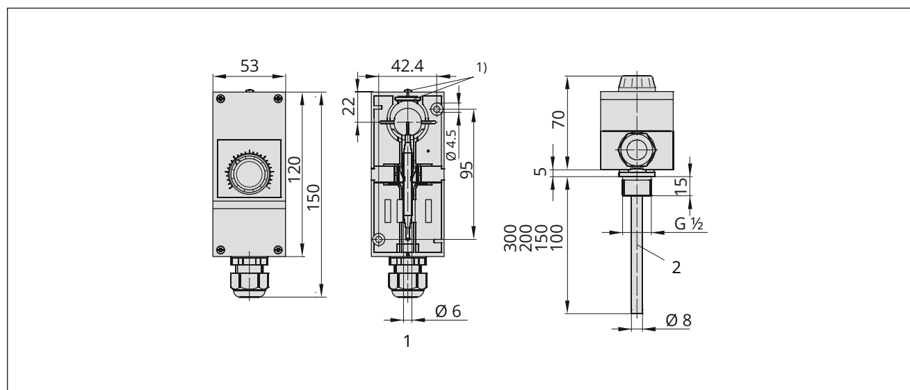
1) Metal plate and screw for fastening the thermostat onto the thermowell (wall mounting) 1 Sensor 2 Thermowell (accessories)
