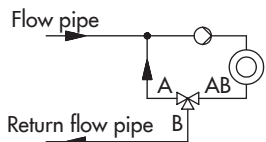
Fig. 4: Typical installations
