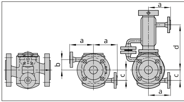
Fig. 9: Type 3241 with heating jacket, nominal size DN 150/NPS 6 and larger · With insulating section or bellows seal (right)
