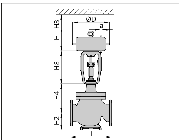
Fig. 4: Type 3241-1 (Type 3271 Pneumatic Actuator) in nominal size DN 200/NPS 8 and larger
